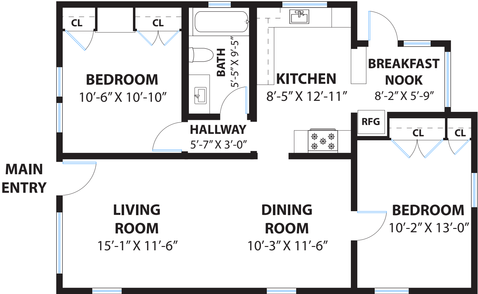
MAIN LEVEL
