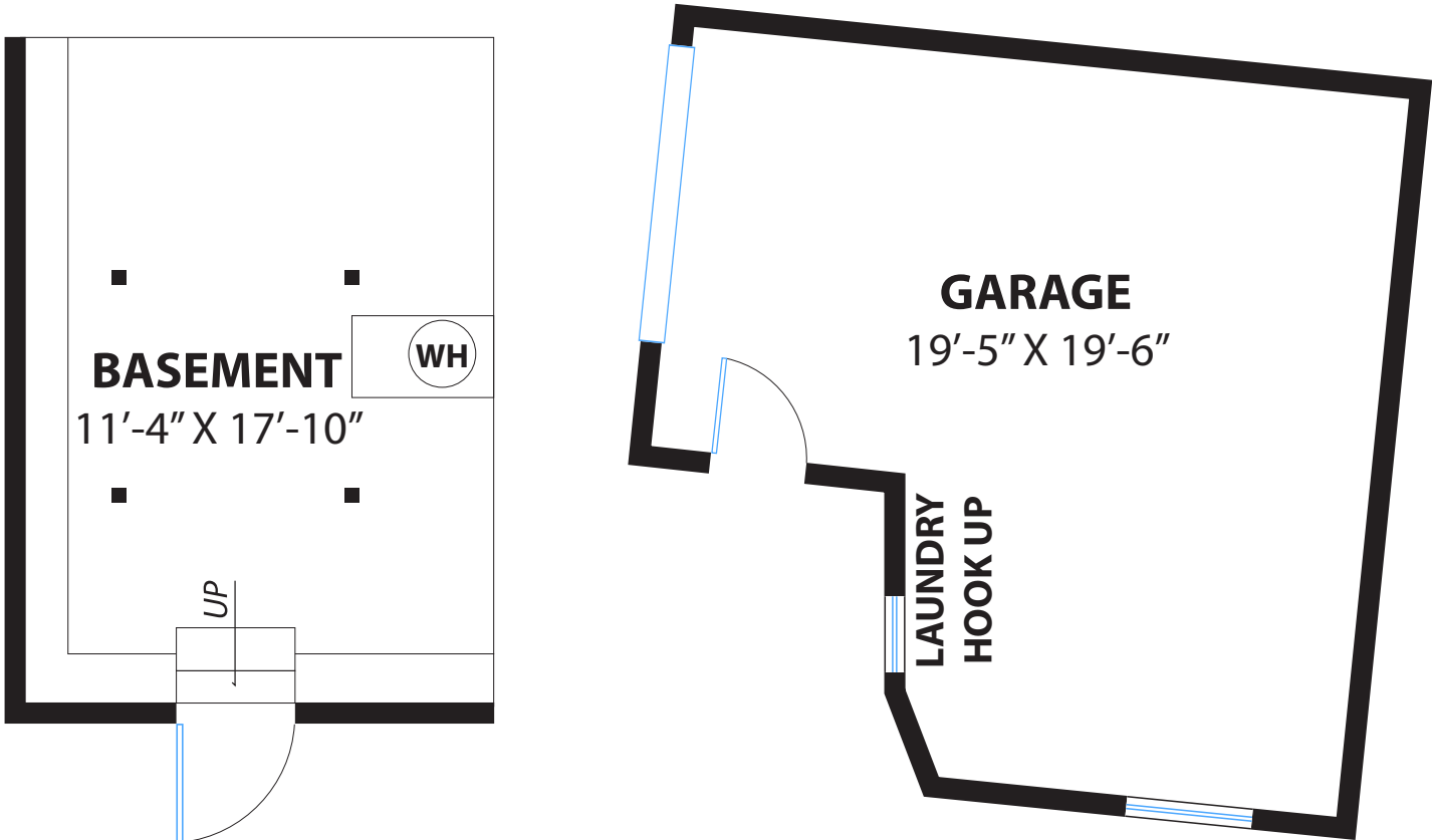
LOWER LEVEL
